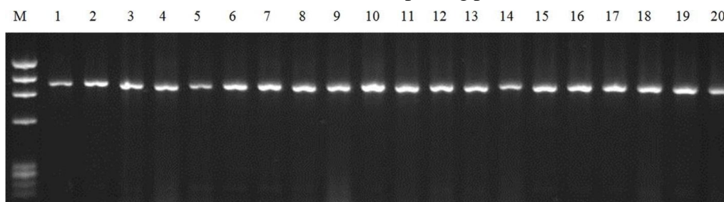
Fig. 1. PCR results of the selected clones after panning. 950 bp bands were obtained for each clone (Lanes 1-20). M: \Phi X174DNA marker.
